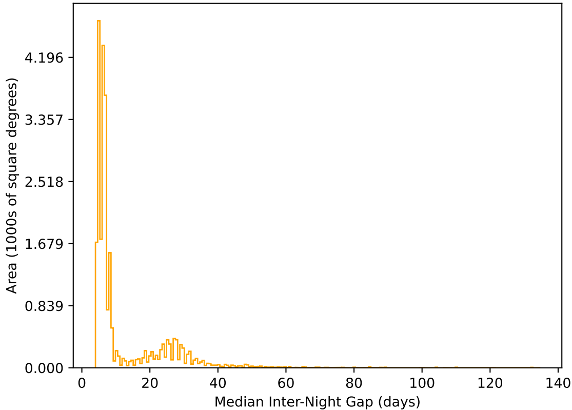
too_elab_heavy_r64_d3_griz_v3.4_10yrs All sky r band: Median Inter-Night Gap
