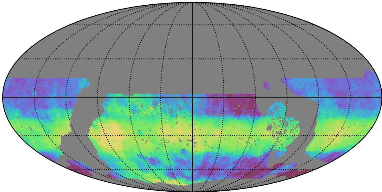
too_elab_heavy_r64_d3_griz_v3.4_10yrs WFD z band: Median HA
