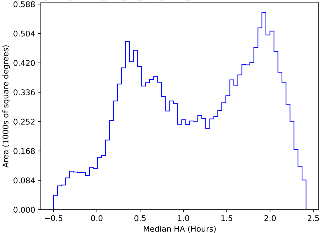
too_elab_heavy_r64_d3_griz_v3.4_10yrs WFD z band: Median HA
