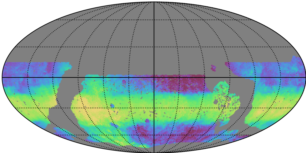
too_elab_heavy_r64_d3_griz_v3.4_10yrs WFD y band: Median HA
