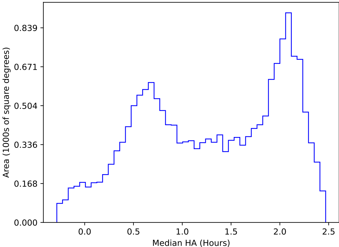
too_elab_heavy_r64_d3_griz_v3.4_10yrs WFD y band: Median HA
