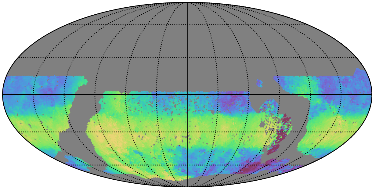
too_elab_heavy_r64_d3_griz_v3.4_10yrs WFD u band: Median HA
