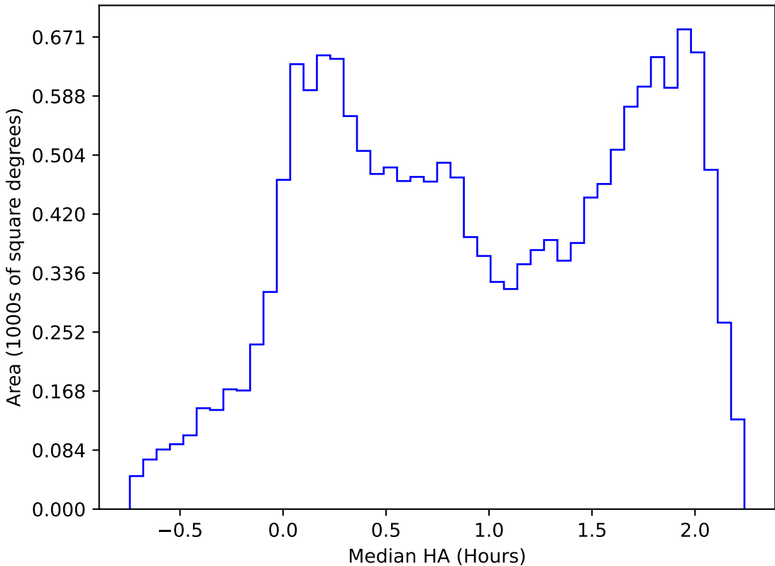
too_elab_heavy_r64_d3_griz_v3.4_10yrs WFD r band: Median HA
