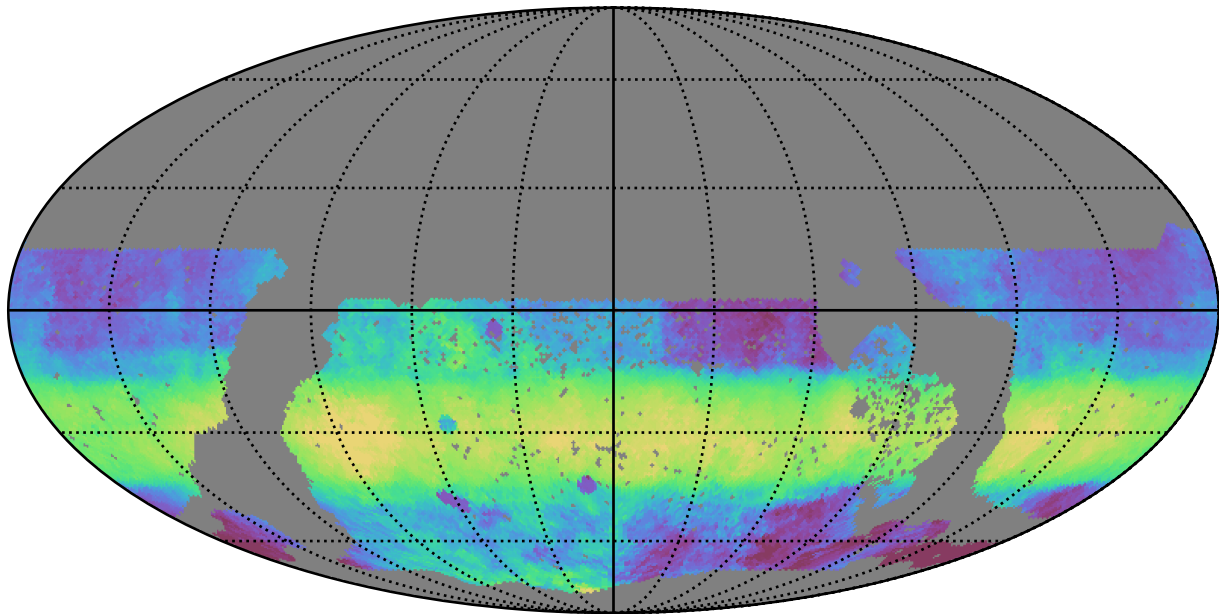
too_elab_heavy_r64_d3_griz_v3.4_10yrs WFD i band: Median HA
