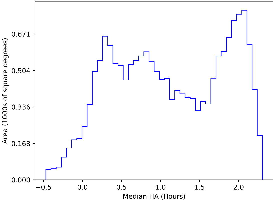
too_elab_heavy_r64_d3_griz_v3.4_10yrs WFD i band: Median HA
