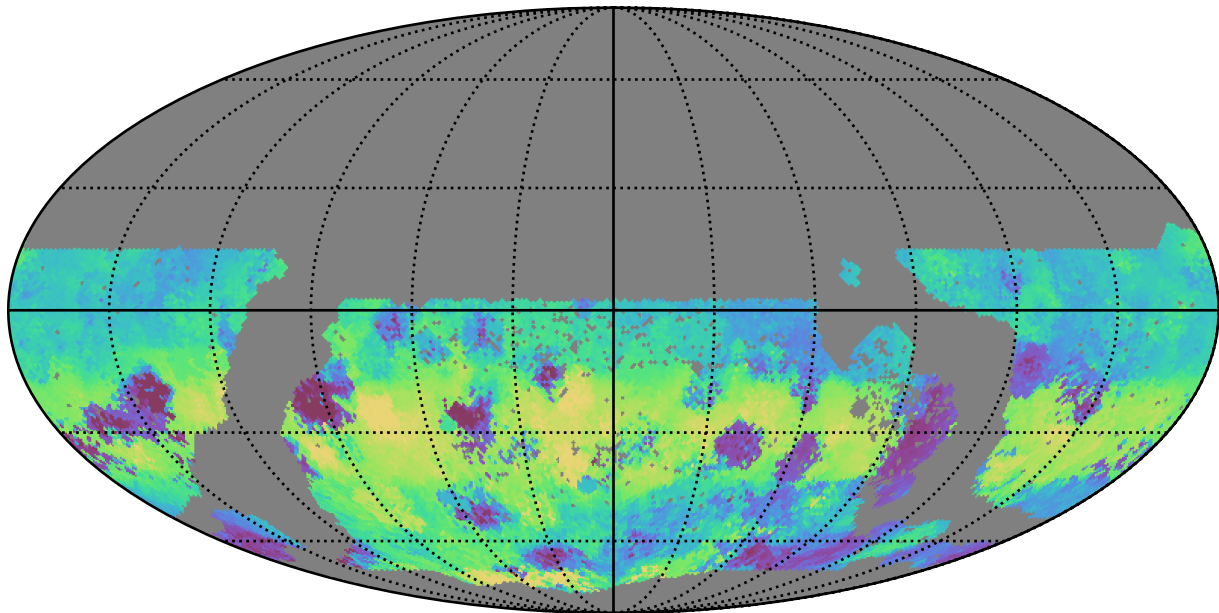
too_elab_heavy_r64_d3_griz_v3.4_10yrs WFD g band: Median HA
