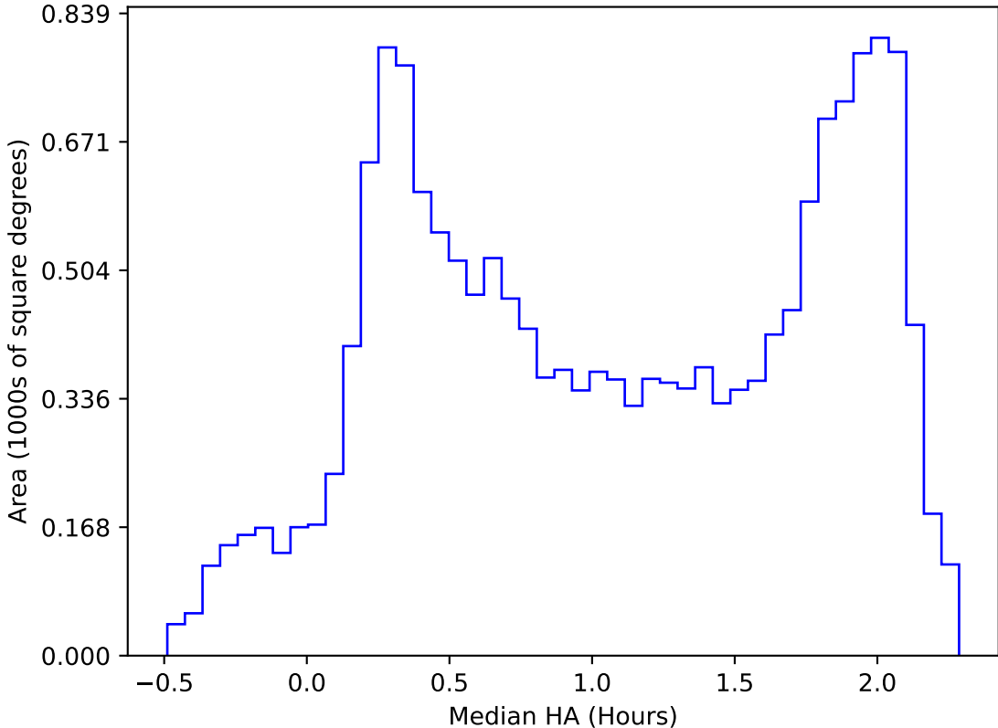
too_elab_heavy_r64_d3_griz_v3.4_10yrs WFD all bands: Median HA
