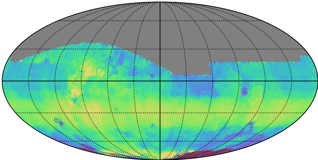
too_elab_heavy_r64_d3_griz_v3.4_10yrs All sky z band: Median HA
