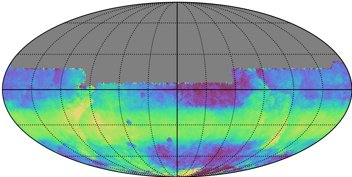
too_elab_heavy_r64_d3_griz_v3.4_10yrs All sky y band: Median HA
