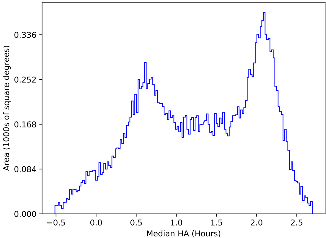
too_elab_heavy_r64_d3_griz_v3.4_10yrs All sky y band: Median HA
