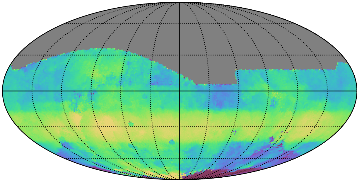
too_elab_heavy_r64_d3_griz_v3.4_10yrs All sky r band: Median HA
