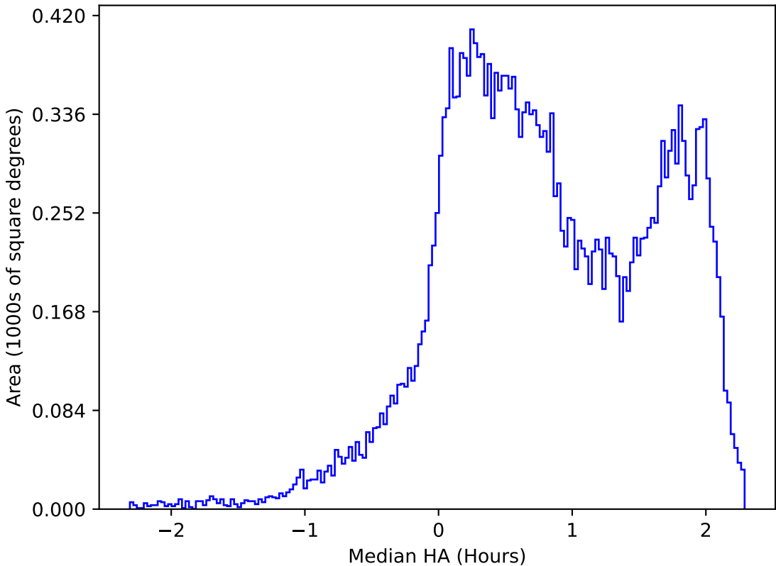
too_elab_heavy_r64_d3_griz_v3.4_10yrs All sky r band: Median HA
