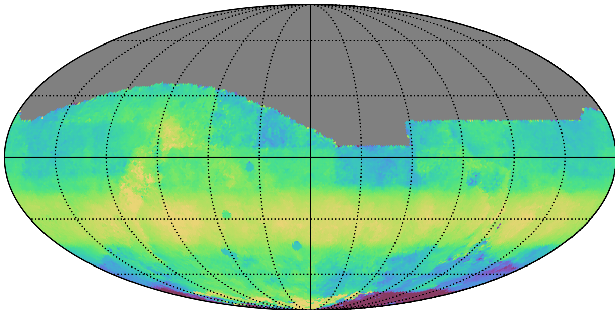
too_elab_heavy_r64_d3_griz_v3.4_10yrs All sky i band: Median HA
