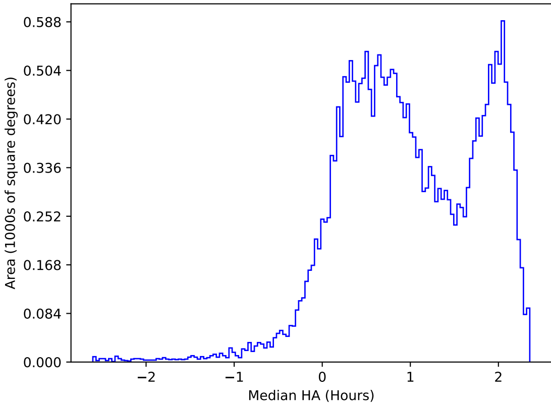
too_elab_heavy_r64_d3_griz_v3.4_10yrs All sky i band: Median HA
