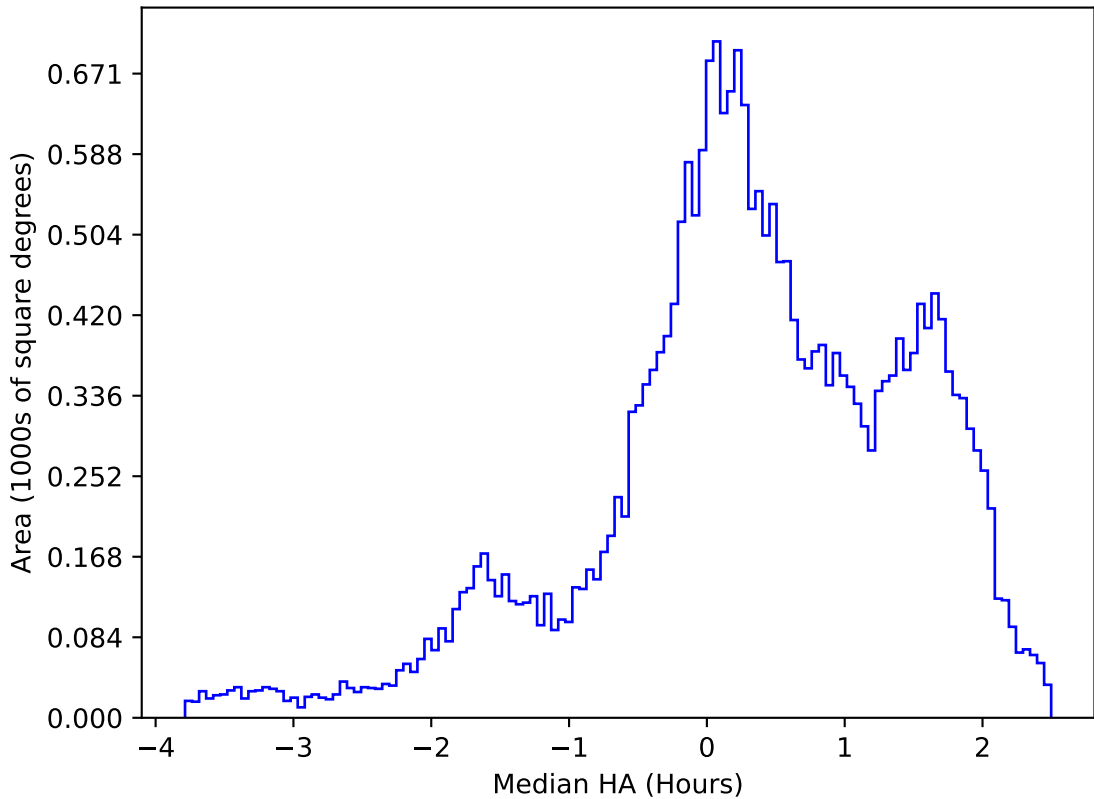
too_elab_heavy_r64_d3_griz_v3.4_10yrs All sky g band: Median HA
