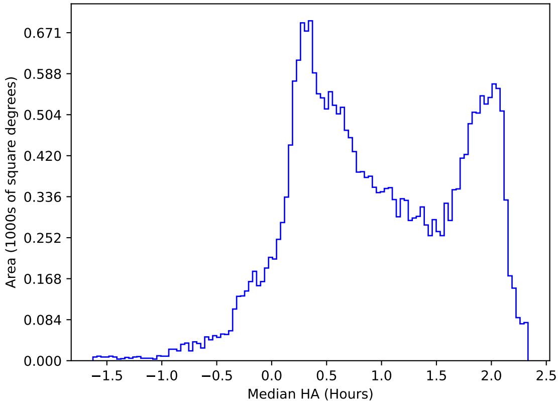
too_elab_heavy_r64_d3_griz_v3.4_10yrs All sky all bands: Median HA
