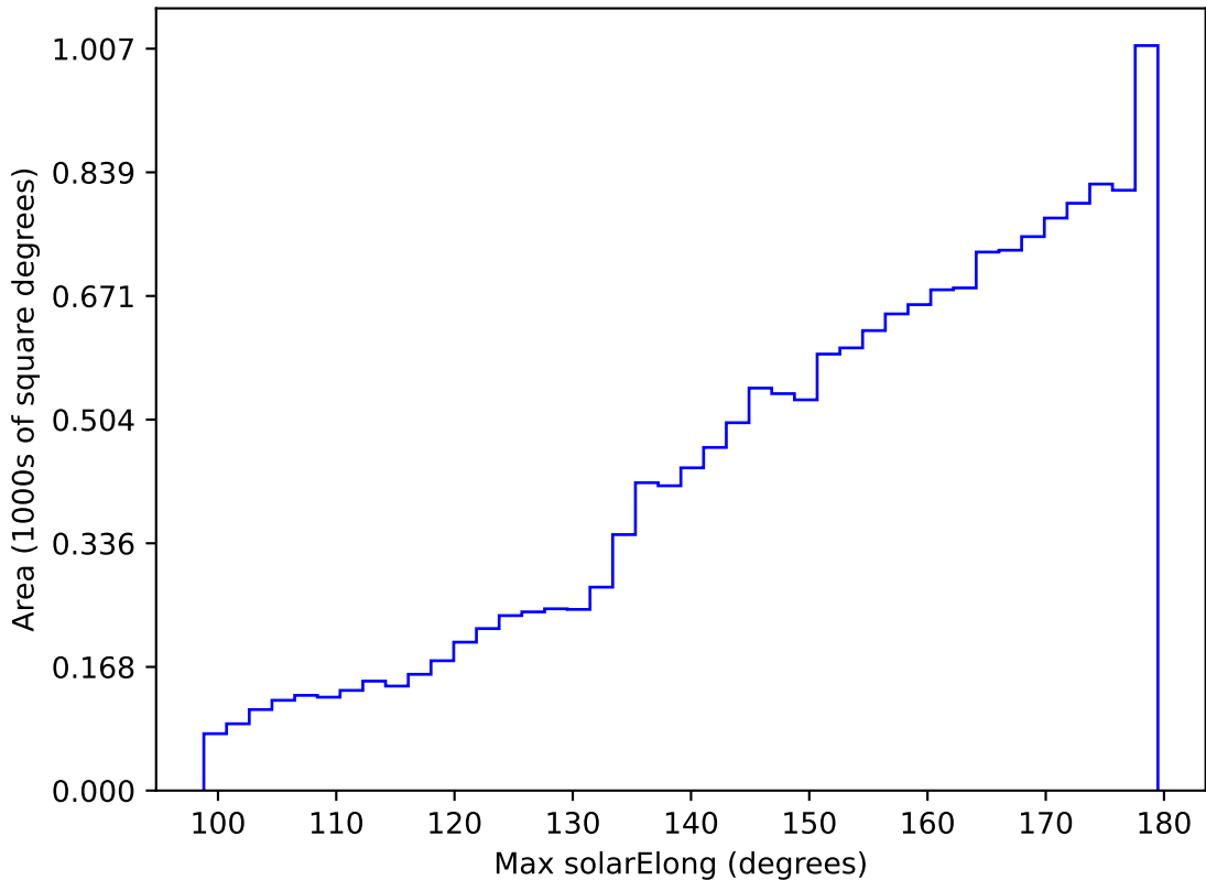
too_elab_heavy_r64_d3_griz_v3.4_10yrs WFD r band: Max solarElong
