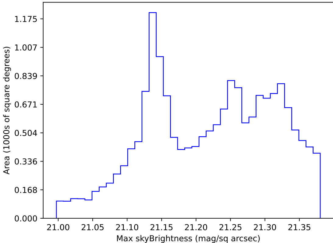
too_elab_heavy_r64_d3_griz_v3.4_10yrs WFD r band: Max skyBrightness
