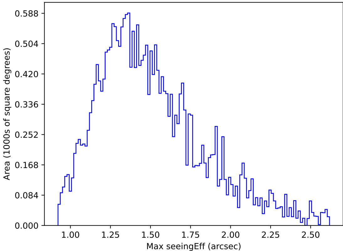
too_elab_heavy_r64_d3_griz_v3.4_10yrs Yr 1 g band: Max seeingEff
