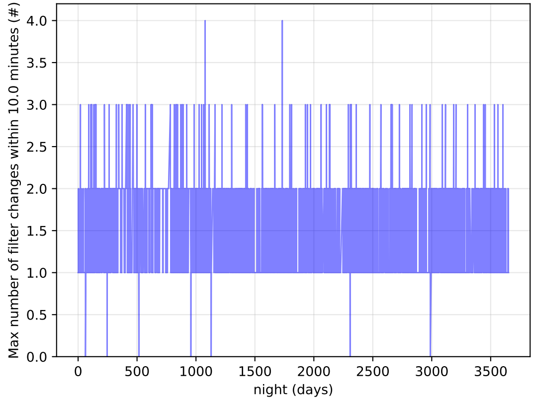
too_elab_heavy_r64_d3_griz_v3.4_10yrs Per Night: Max number of filter changes within 10.0 minutes
