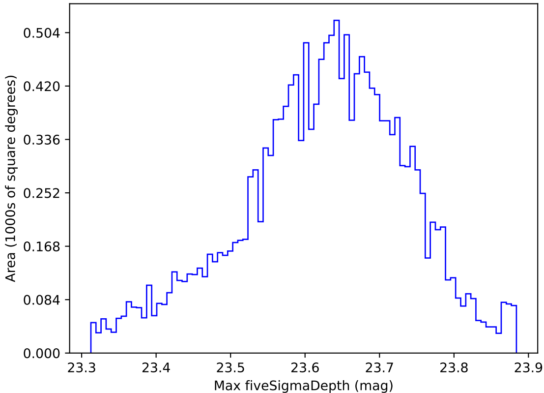
too_elab_heavy_r64_d3_griz_v3.4_10yrs WFD z band: Max fiveSigmaDepth
