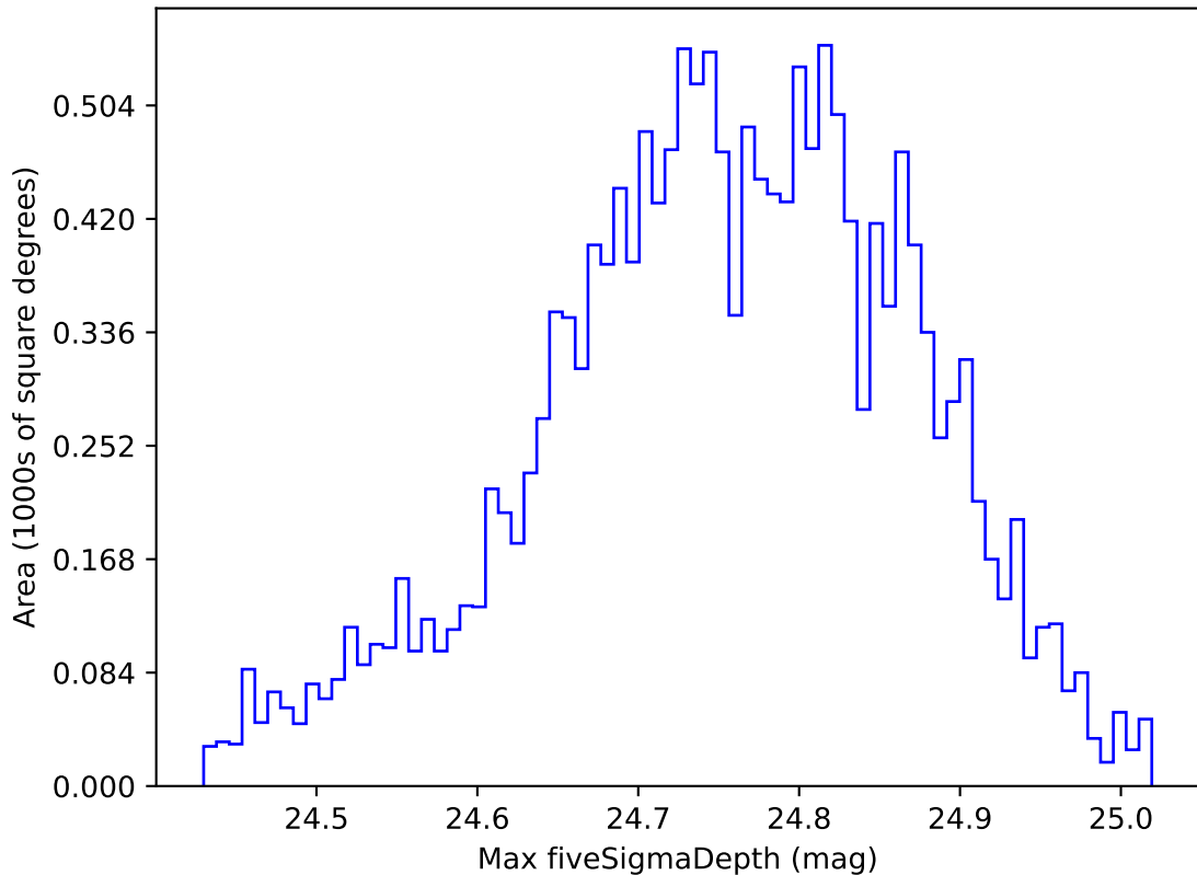
too_elab_heavy_r64_d3_griz_v3.4_10yrs WFD r band: Max fiveSigmaDepth
