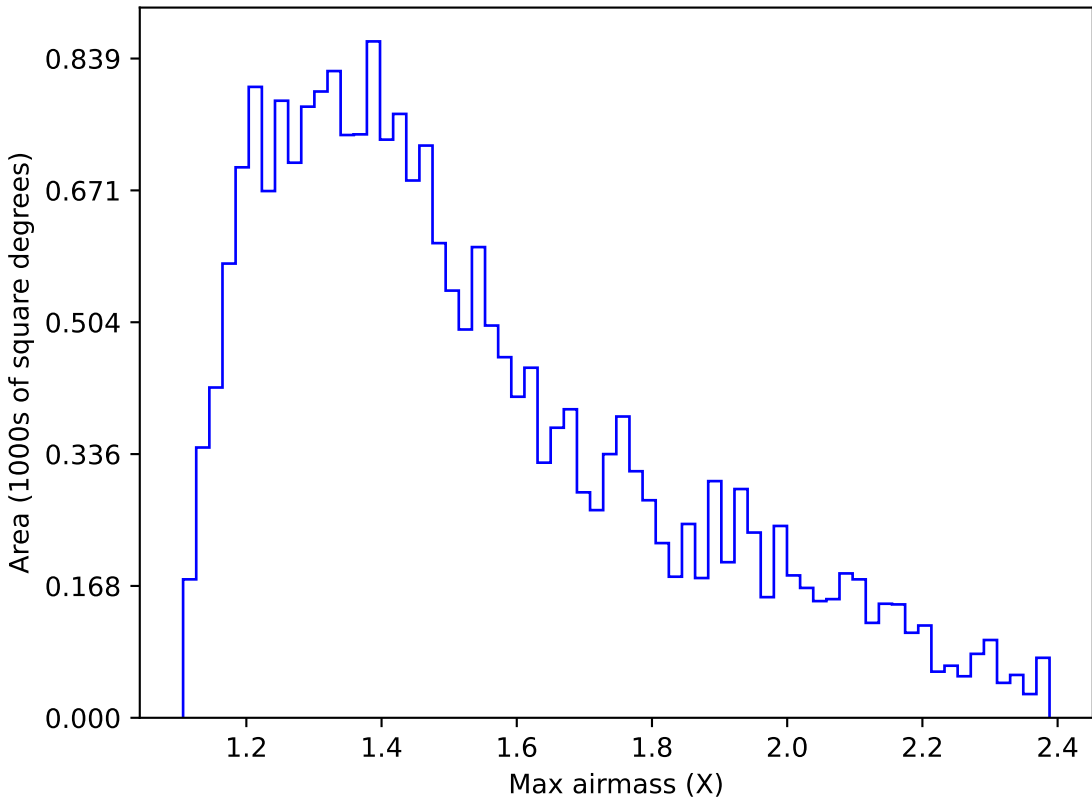
too_elab_heavy_r64_d3_griz_v3.4_10yrs Yr 1 u band: Max airmass
