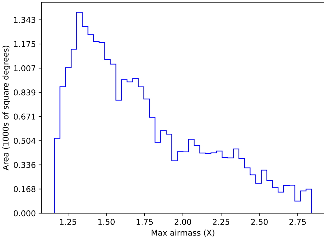
too_elab_heavy_r64_d3_griz_v3.4_10yrs Yr 1 i band: Max airmass
