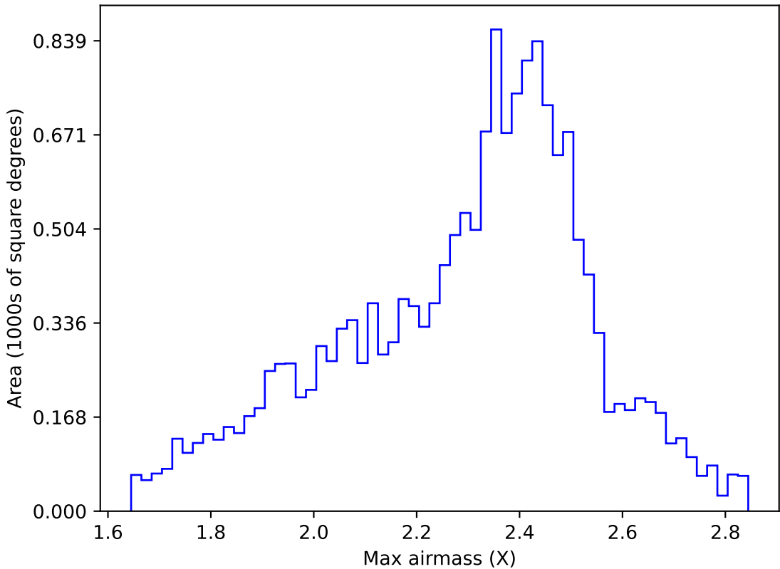
too_elab_heavy_r64_d3_griz_v3.4_10yrs WFD r band: Max airmass
