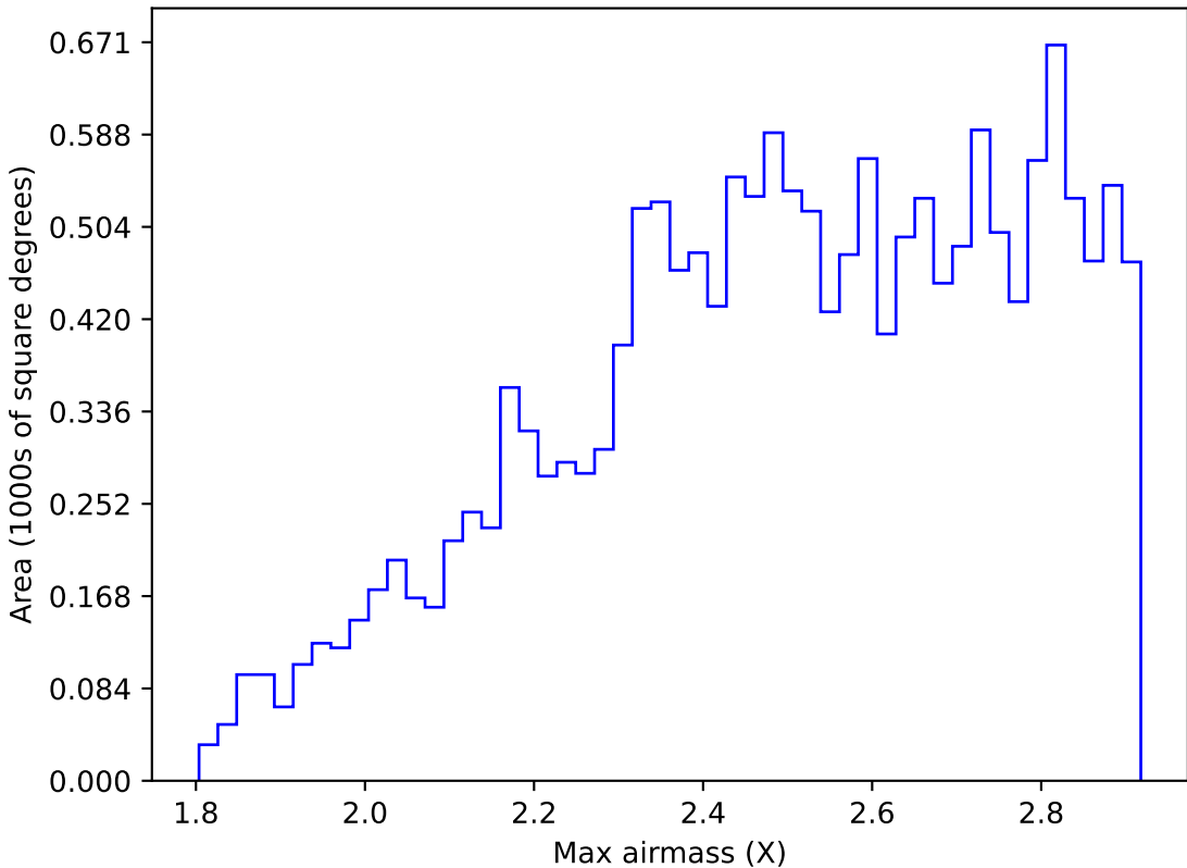
too_elab_heavy_r64_d3_griz_v3.4_10yrs WFD i band: Max airmass
