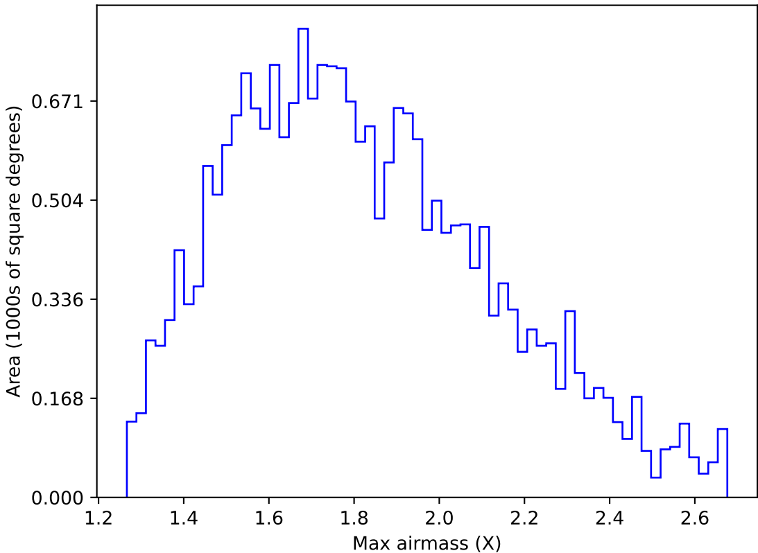
too_elab_heavy_r64_d3_griz_v3.4_10yrs All sky u band: Max airmass
