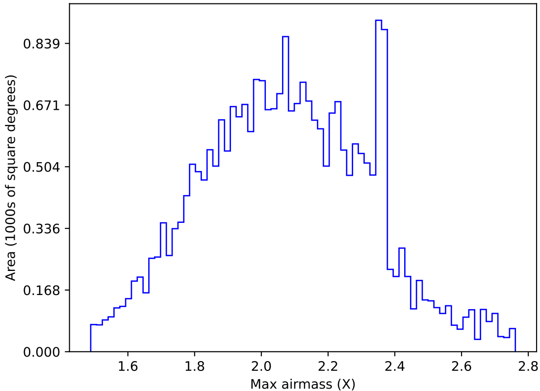
too_elab_heavy_r64_d3_griz_v3.4_10yrs All sky g band: Max airmass
