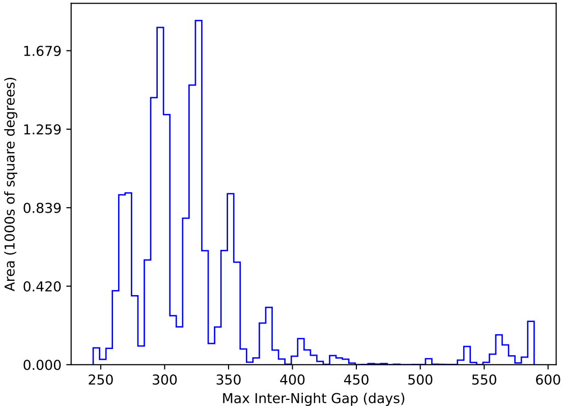
too_elab_heavy_r64_d3_griz_v3.4_10yrs WFD y band: Max Inter-Night Gap
