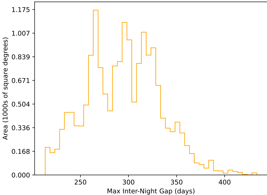
too_elab_heavy_r64_d3_griz_v3.4_10yrs WFD r band: Max Inter-Night Gap
