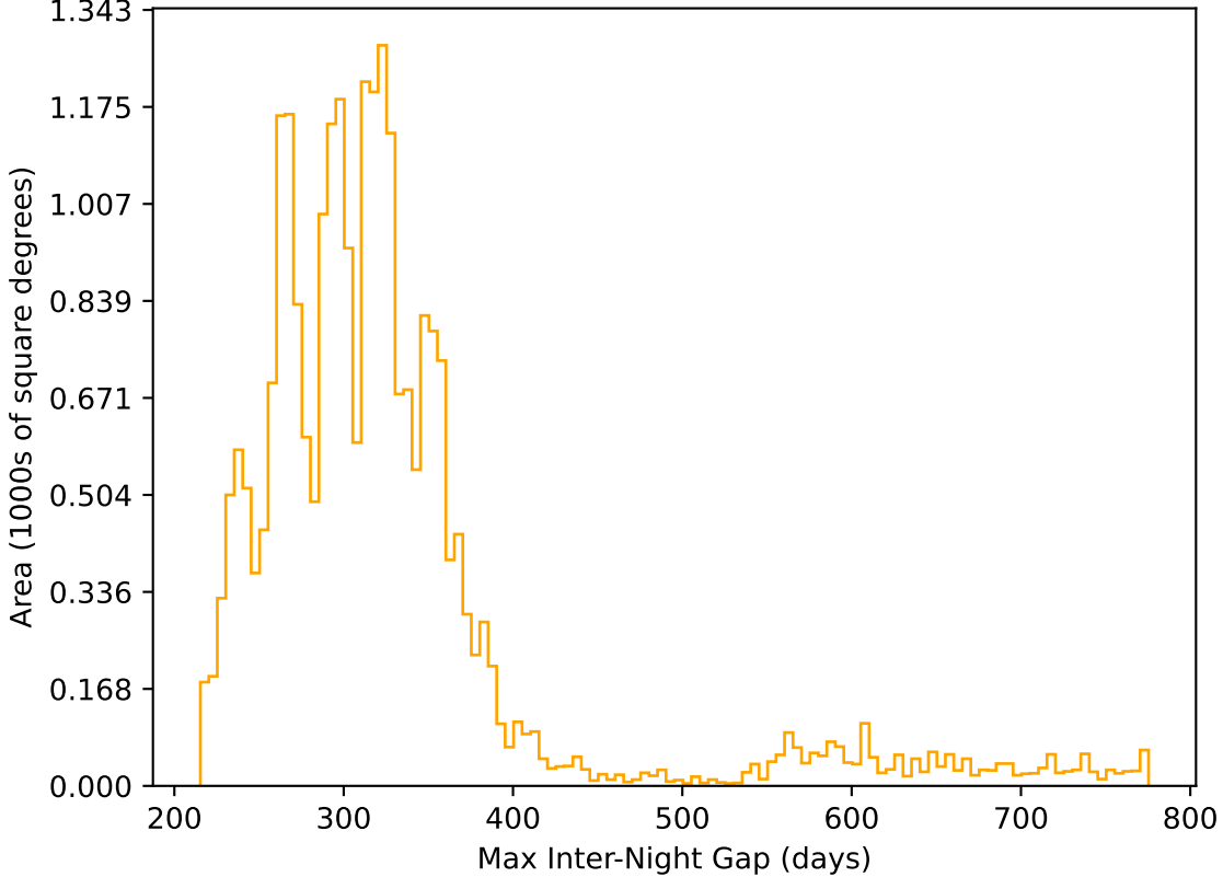
too_elab_heavy_r64_d3_griz_v3.4_10yrs All sky r band: Max Inter-Night Gap
