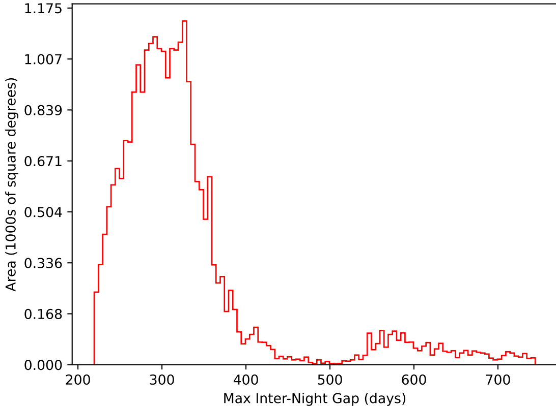
too_elab_heavy_r64_d3_griz_v3.4_10yrs All sky i band: Max Inter-Night Gap
