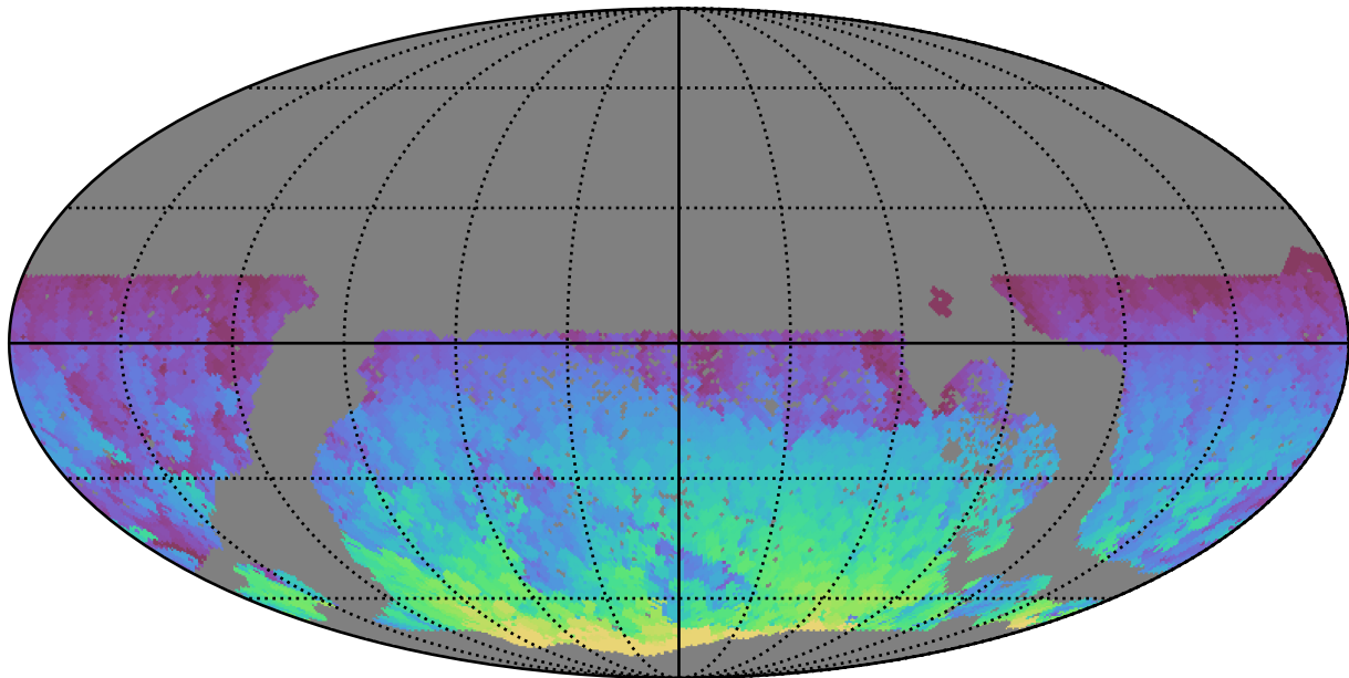
too_elab_heavy_r64_d3_griz_v3.4_10yrs WFD z band: Max HA
