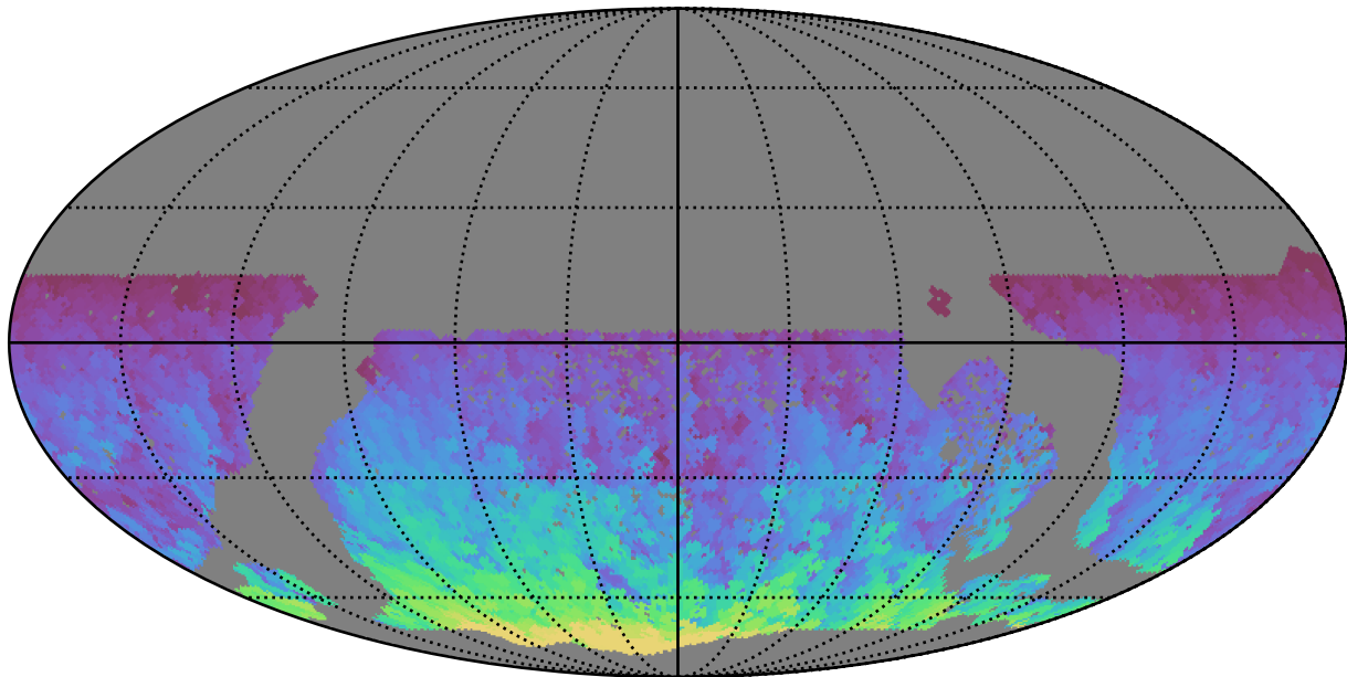
too_elab_heavy_r64_d3_griz_v3.4_10yrs WFD y band: Max HA
