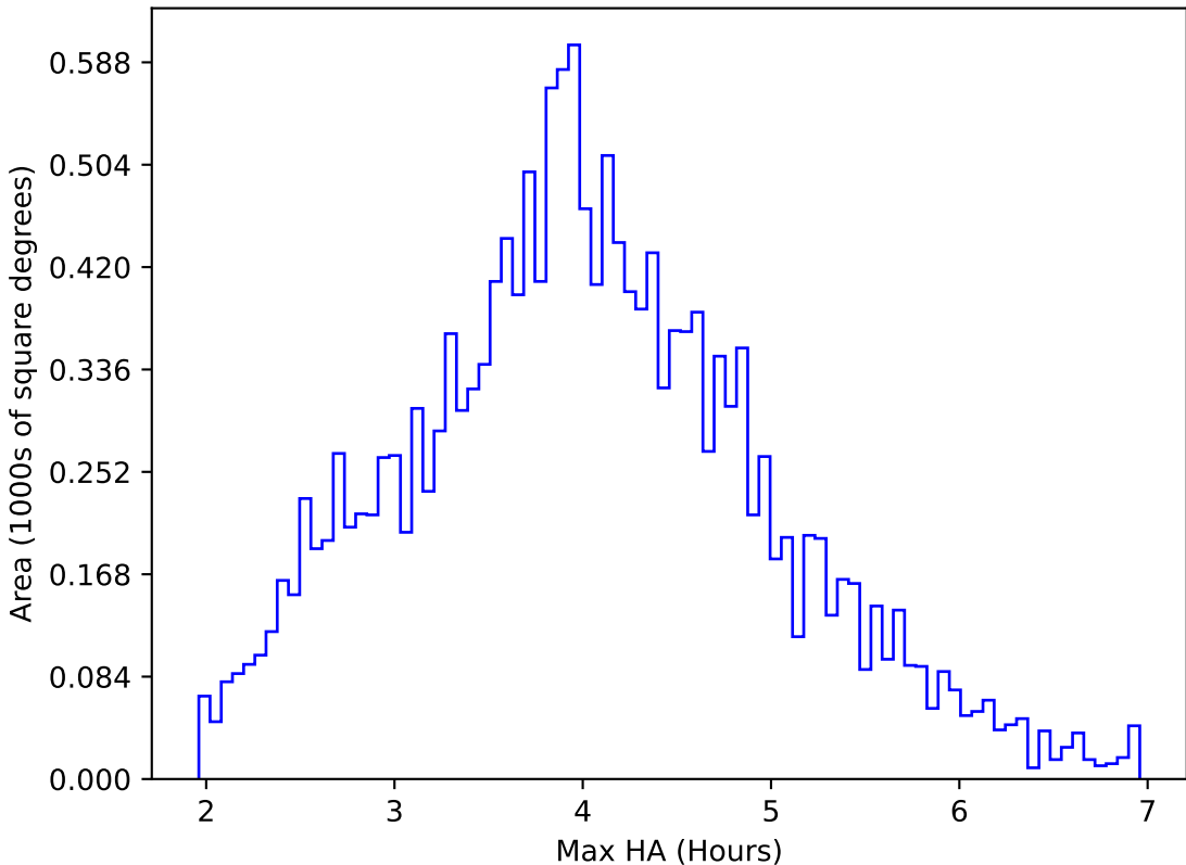
too_elab_heavy_r64_d3_griz_v3.4_10yrs WFD u band: Max HA
