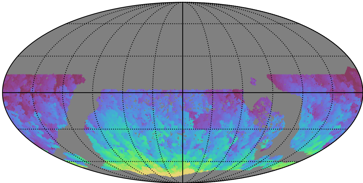
too_elab_heavy_r64_d3_griz_v3.4_10yrs WFD r band: Max HA
