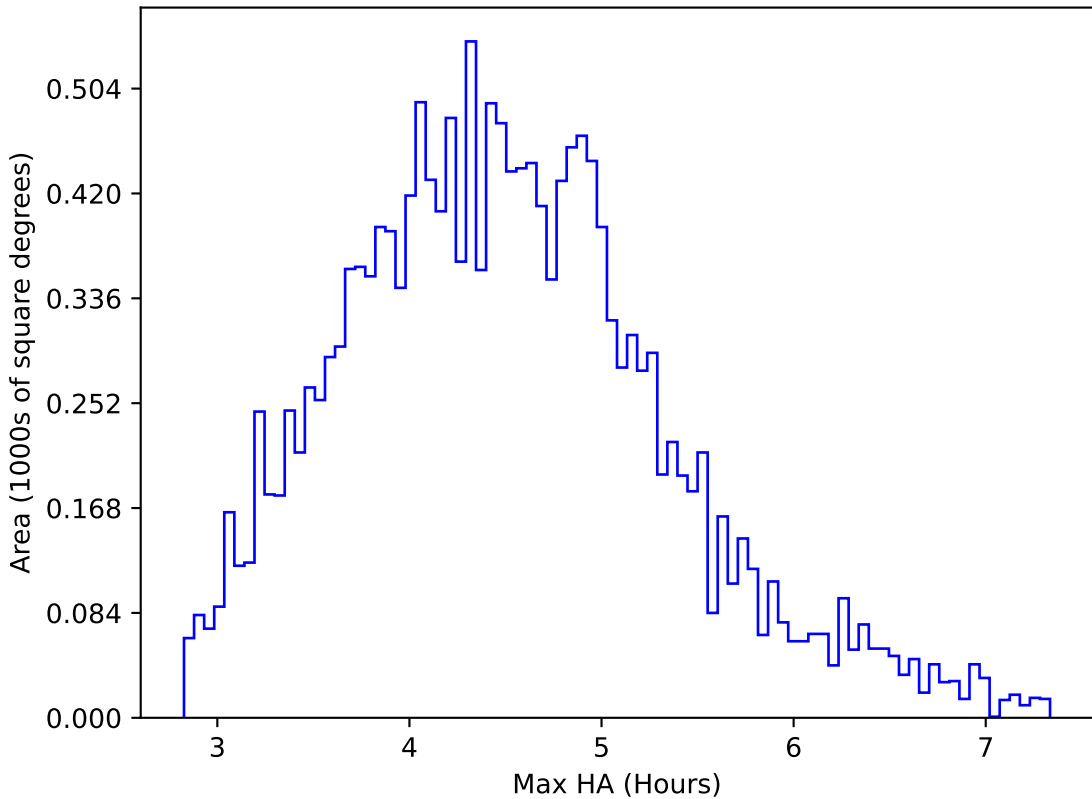
too_elab_heavy_r64_d3_griz_v3.4_10yrs WFD r band: Max HA
