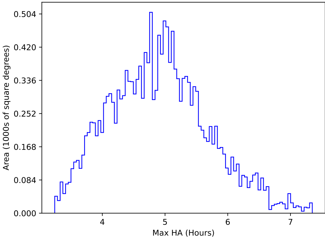
too_elab_heavy_r64_d3_griz_v3.4_10yrs WFD i band: Max HA
