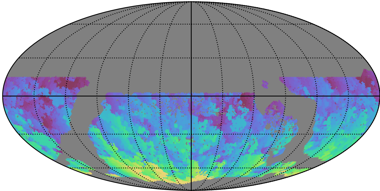
too_elab_heavy_r64_d3_griz_v3.4_10yrs WFD g band: Max HA
