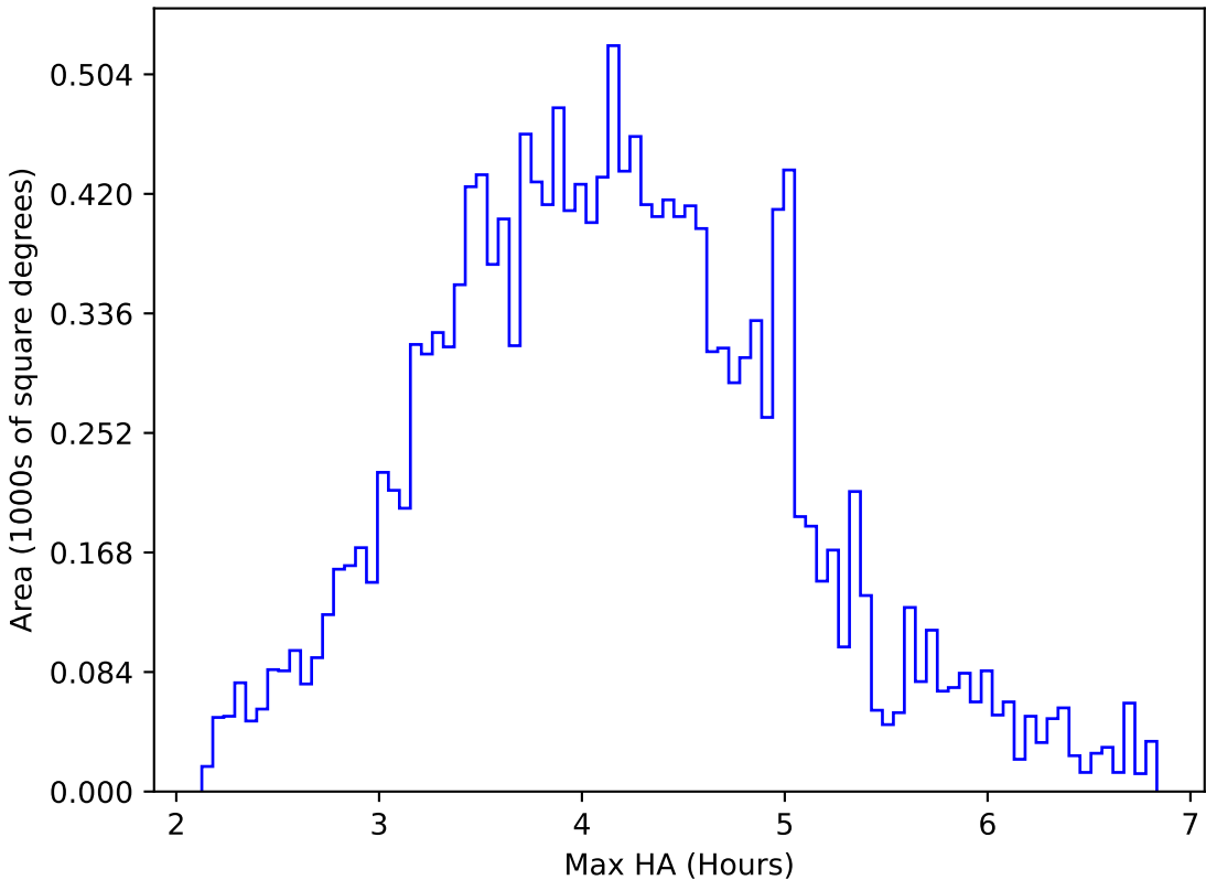
too_elab_heavy_r64_d3_griz_v3.4_10yrs WFD g band: Max HA
