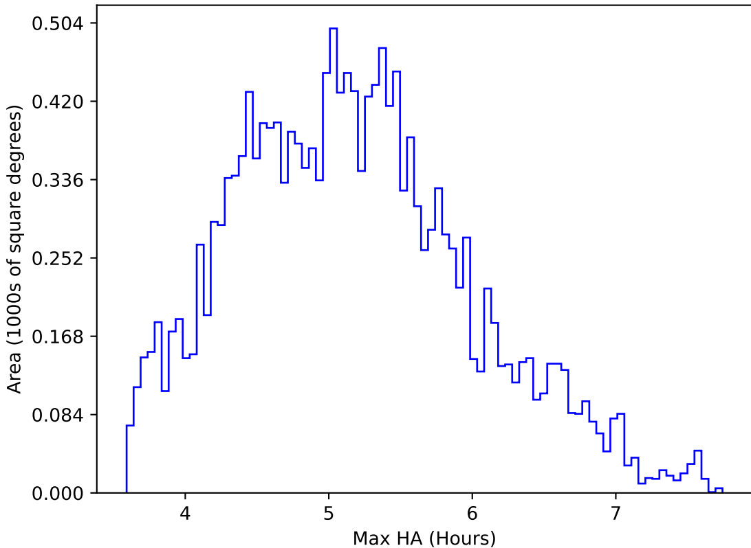
too_elab_heavy_r64_d3_griz_v3.4_10yrs WFD all bands: Max HA
