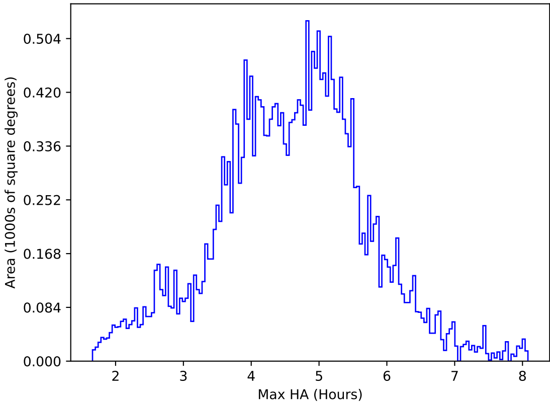
too_elab_heavy_r64_d3_griz_v3.4_10yrs All sky z band: Max HA
