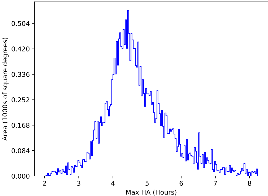
too_elab_heavy_r64_d3_griz_v3.4_10yrs All sky y band: Max HA
