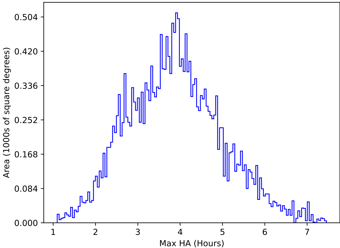
too_elab_heavy_r64_d3_griz_v3.4_10yrs All sky u band: Max HA
