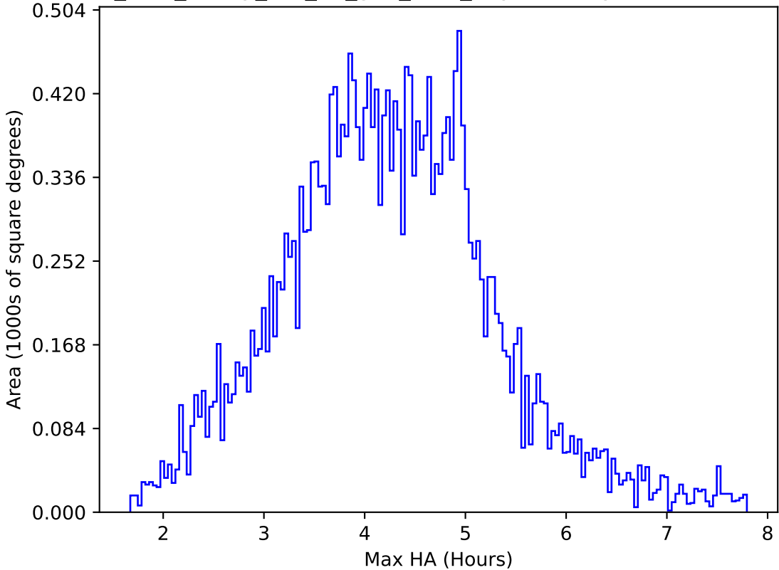
too_elab_heavy_r64_d3_griz_v3.4_10yrs All sky r band: Max HA
