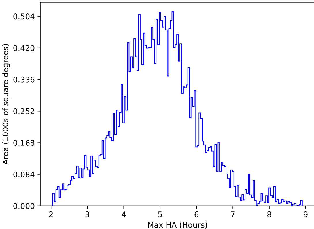
too_elab_heavy_r64_d3_griz_v3.4_10yrs All sky all bands: Max HA
